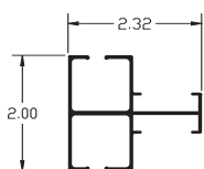
2" Divider ITEM NO. SC2138
