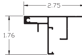
2 Part Large Inner Frame ITEM NO. SC1959
