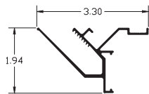
Bleed Fascia Frame ITEM NO. SC2092
