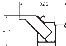
1-1/2" Tension Frame Cover ITEM NO. SC2084
