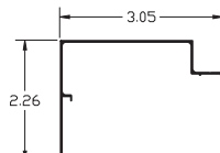
2-1/4" Dual Frame Cover ITEM NO. SC2075
