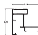
2 Part Extended Frame ITEM NO. SC1941
