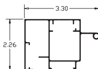
2-1/4" Retainer ITEM NO. SC2045
