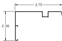
2-3/8" Retro Frame Cover ITEM NO. SC2138
