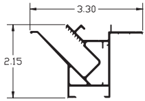
Flat Bleed Retro Frame Cover ITEM NO. SC2121
