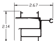
Dual Frame ITEM NO. SC2065
