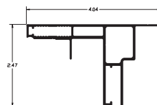
2 Part Large Inner Frame ITEM NO. SC1959
