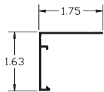
2 Part Extended Frame ITEM NO. SC1955
