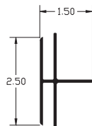
2-1/2" Standard Divider ITEM NO. SC1920
