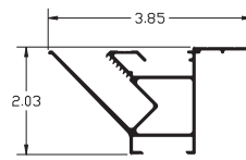
1-1/2" Flat Retro Frame Cover ITEM NO. SC2125
