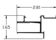
1-1/2" Fascia Frame ITEM NO. SC2094
