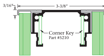
Extended Insert End Cover Part #1698
