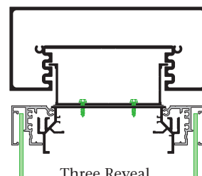
Three Reveal Positions 0", 1/2" & 1"
